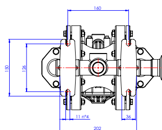
Bottom View Fittings
