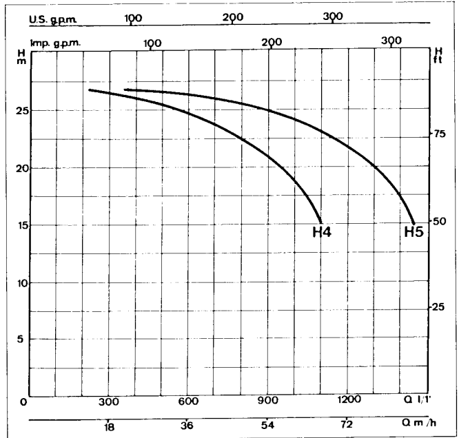
Operating curves at 3000 r.p.m.
